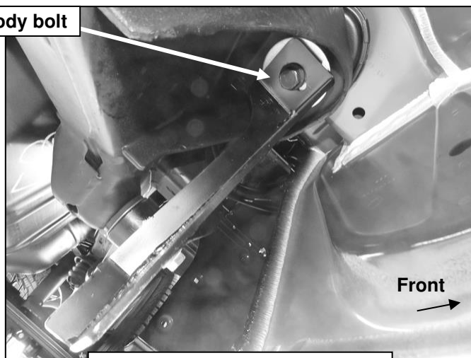
(Fig 10) Driver/left Rear Bracket attached to the rear body mount
