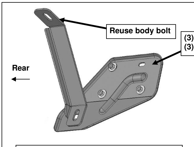
(Fig 10) Reuse body bolt to attach top of Support Bracket to body mount (Driver/left Rear Support Bracket illustrated)
